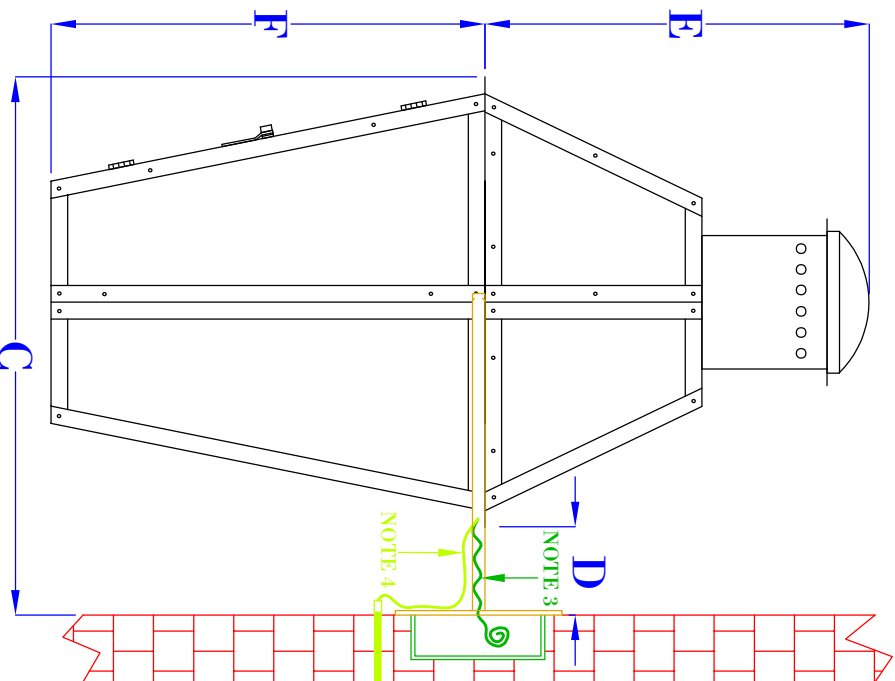
SIDE VIEW (NTS)
