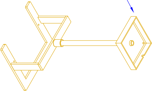
ISOMETRIC VIEW (NTS- BRACKET ONLY)
