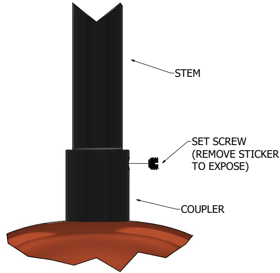
DETAIL A TIGHTEN SET SCREW (BACK SIDE OF BRACKET) AFTER ATTACHING STEM TO COUPLER
