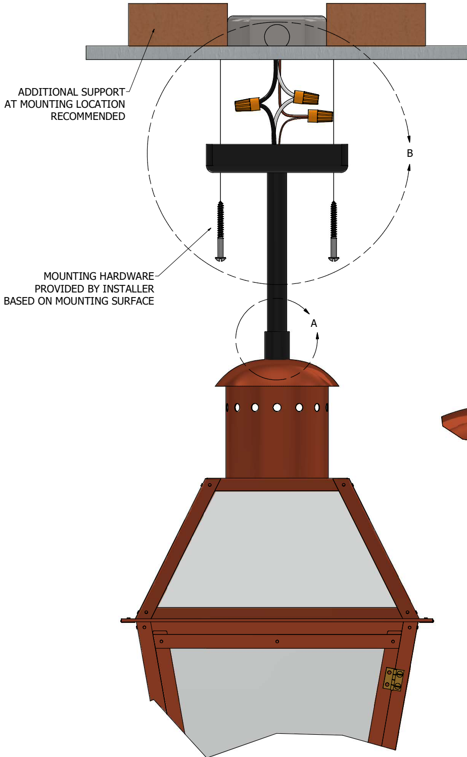
DETAIL A TIGHTEN SET SCREW (BACK SIDE OF BRACKET) AFTER ATTACHING STEM TO COUPLER
