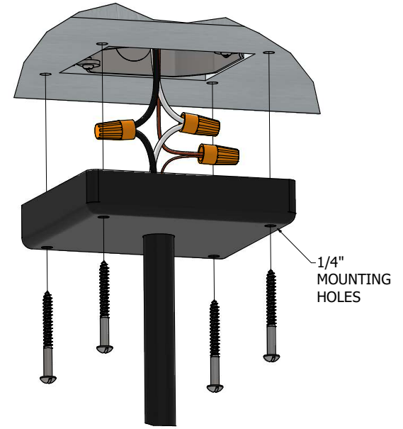
DETAIL B BRACKET MOUNTS DIRECTLY TO CEILING. BRACKET DOES NOT MOUNT TO JUNCTION BOX.
