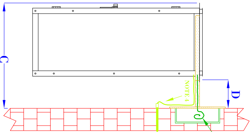
SIDE VIEW (NTS)
