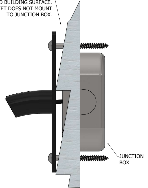
DETAIL A BRACKET INSTALLED
