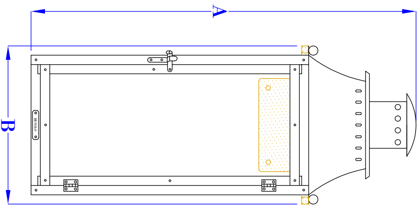
FRONT VIEW (18" VERSION SHOWN)
