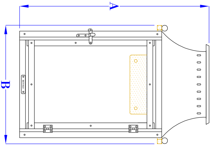
FRONT VIEW (16" VERSION SHOWN)
