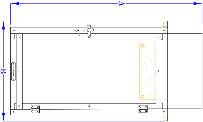
FRONT VIEW (NTS)
