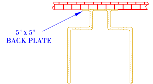
TOP VIEW (NTS- BRACKET ONLY)
