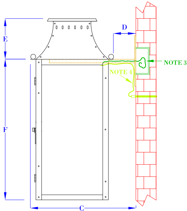
SIDE VIEW (NTS)
