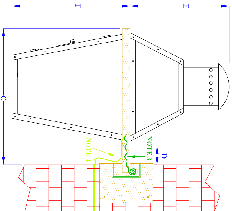
SIDE VIEW (NTS)
