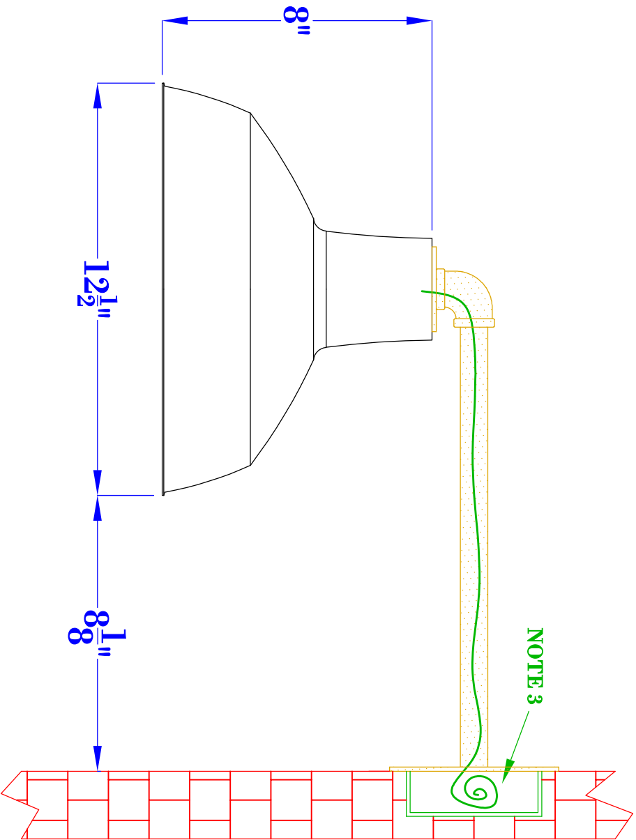
SIDE VIEW (NTS)
