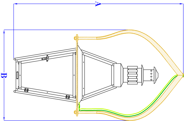
FRONT VIEW (NTS)
