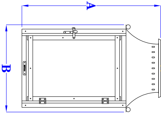
FRONT VIEW (16" VERSION SHOWN)
