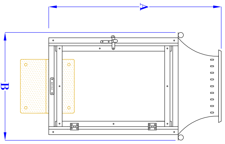
FRONT VIEW (16" VERSION SHOWN)
