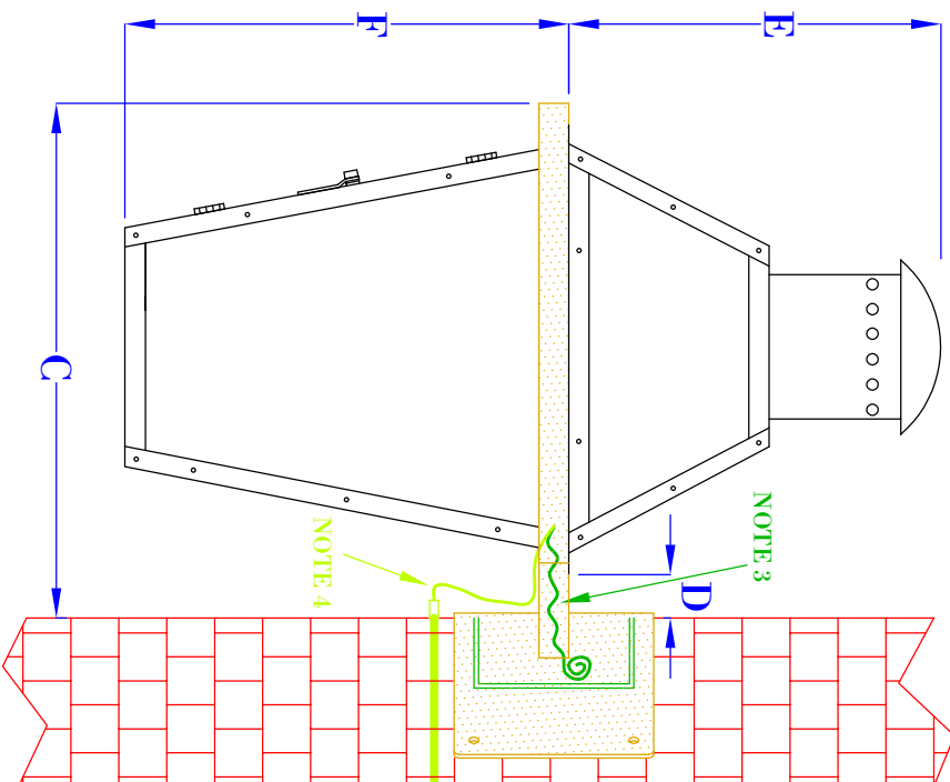
SIDE VIEW (NTS)
